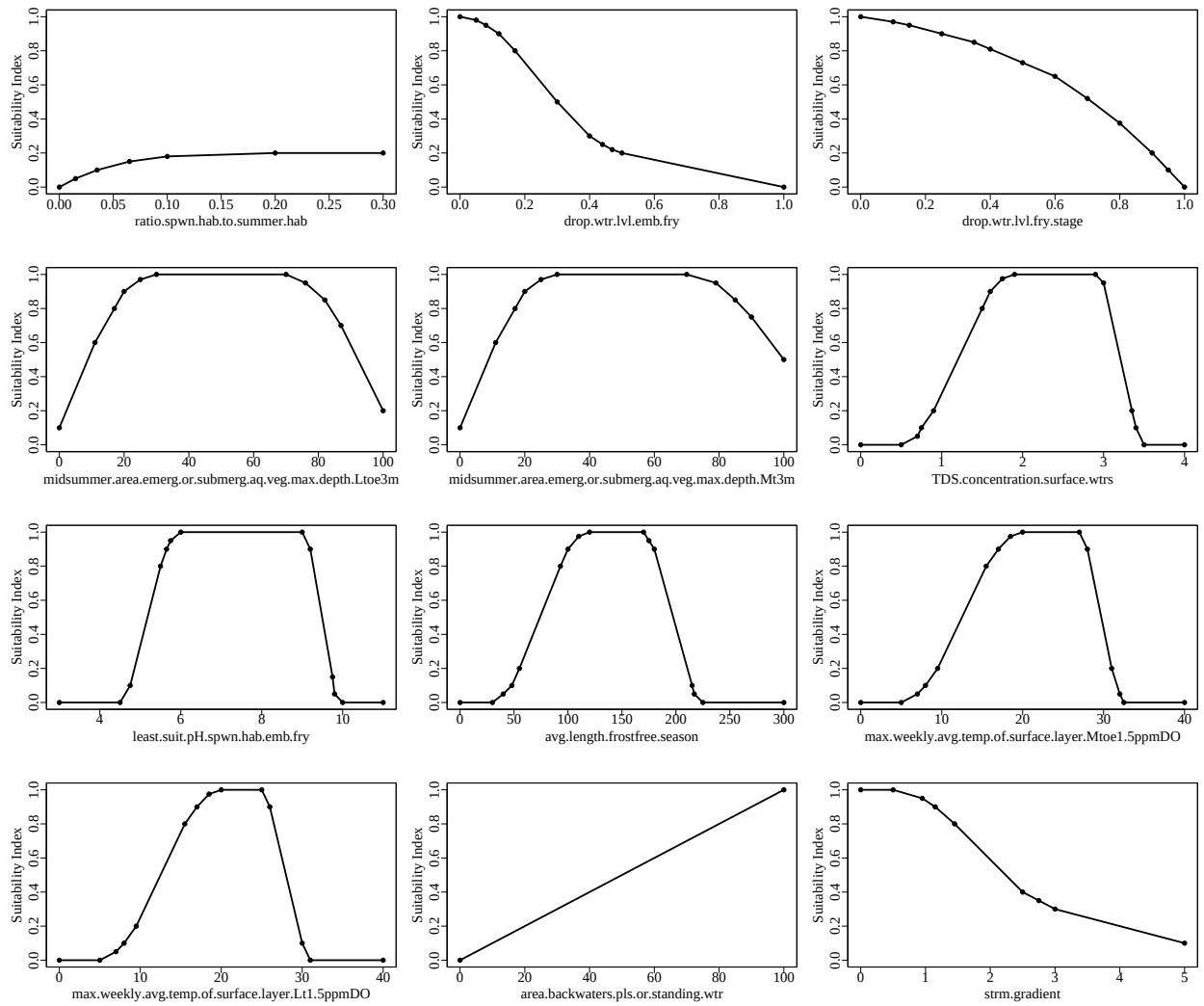
Figure 1. Suitability index graphs for variables included in the northernpikeRivVegD model in ecoest.
